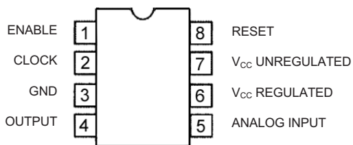
TL507CP
