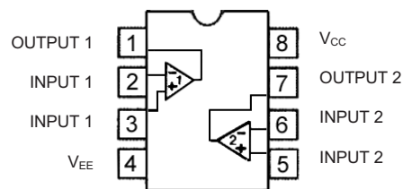
LM833N
