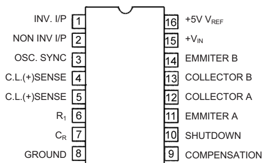
SG3524
