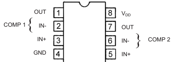
TLC372CP
