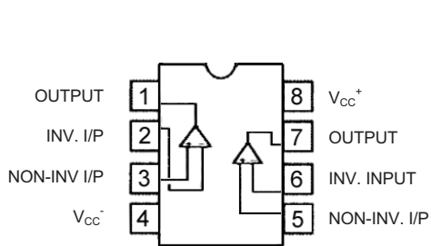
TL082CP
