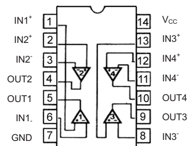
LM3900N
