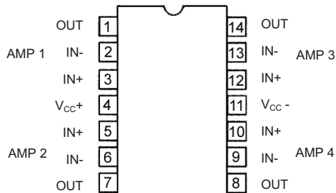
TLC273CP
