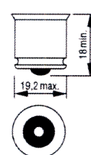
S19S
