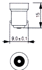
BA9S
