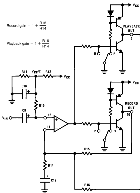
FIGURE 6. Monitor Amplifier
