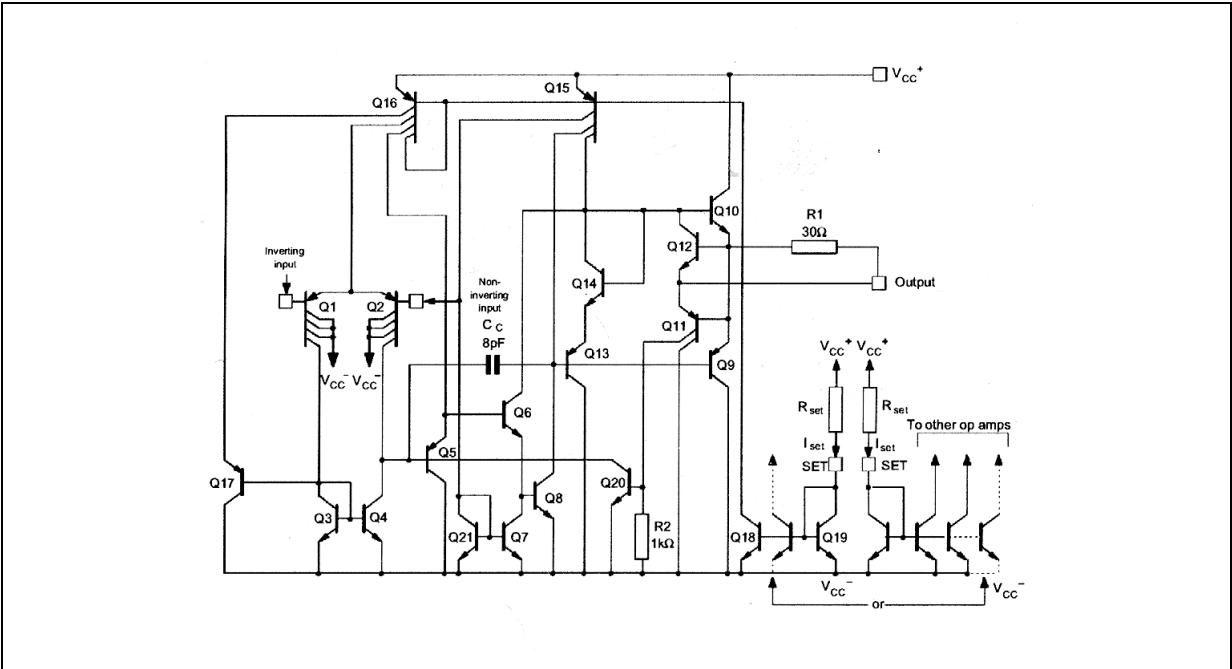
SCHEMATIC DIAGRAM (1/4 LM146)
