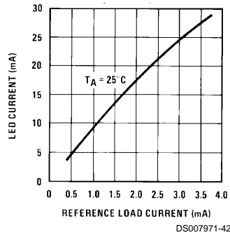
LED Current vs Referenced Loading
