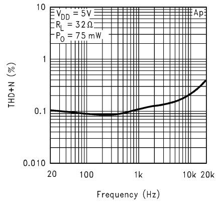
THD+N vs Frequency, 32Ω
