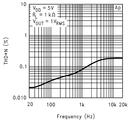
THD+N vs Frequency, 1 kΩ
