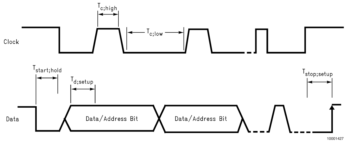
FIGURE 4. I²C Timing Diagram
