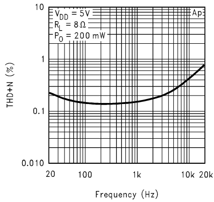
THD+N vs Frequency, 8Ω
