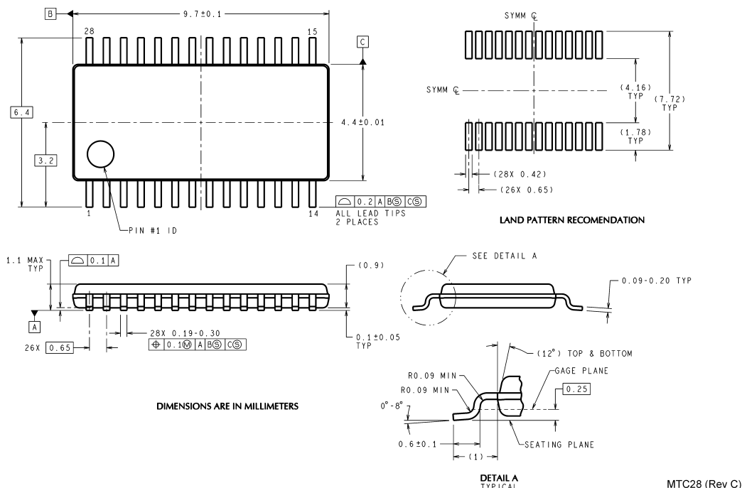
28-Lead TSSOP Order Number LM4832MT NS Package Number MTC28
