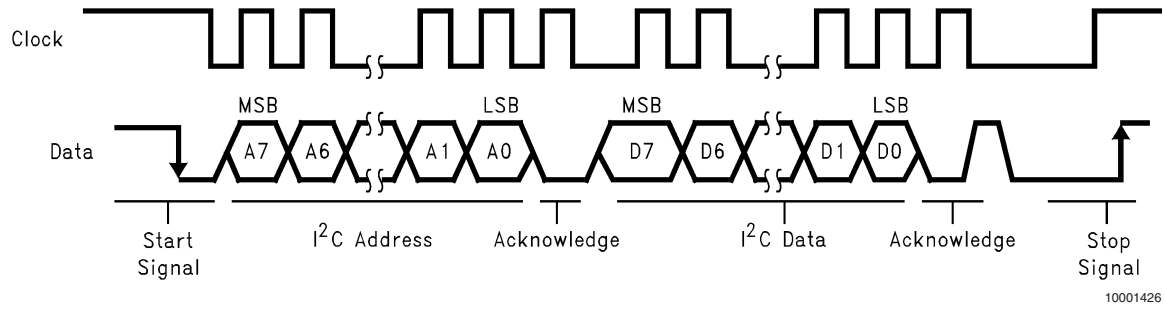
FIGURE 3. I²C Bus Format
