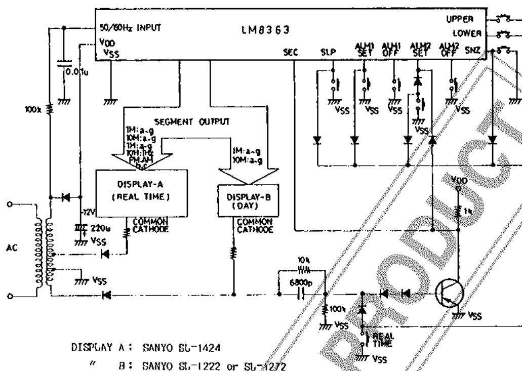
Sample Application Circuit 2: 6-digit display (Current time + date, 12-hour system)
